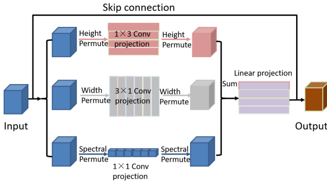
Fig. 3. Illustration of the proposed Conv-Permute module. The proposed Conv-Permute module first encodes the spatial-spectral features along the height, width, and spectral dimensions, respectively. The extracted features are then aggregated utilizing elementwise addition and a fully connected layer.
